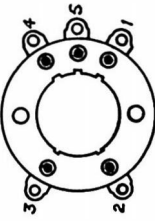
5AA & 7AA (ACORN VALVES)
