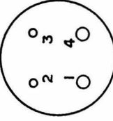
AMERICAN FOUR PIN (UX4)
