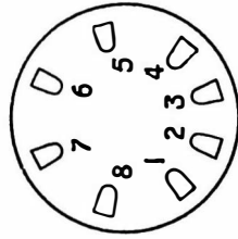
'P' TYPE BASE (B5C)
