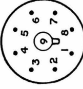
AMERICAN OCTAL (B8B or B8G)
